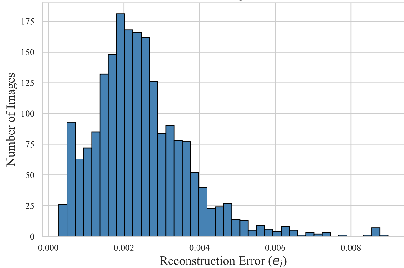
CAE: Distribution of Per-Image Reconstruction Error
